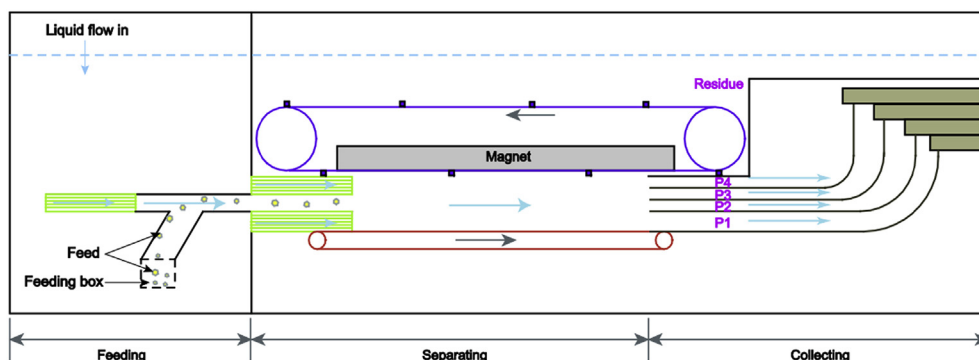
Fig. 7. Schematic of magnetic density separator [154].
