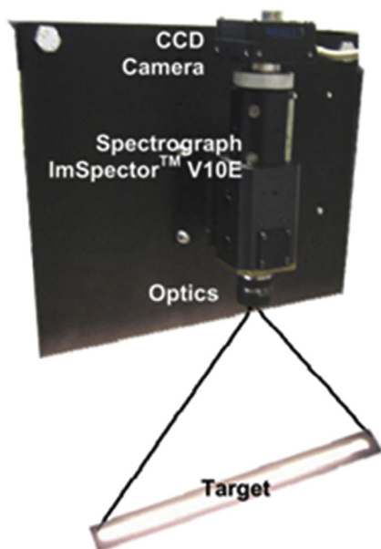
Fig. 8. Hyper spectral Imaging (HSI) based acquisition device to collect secondary plastic particle flow streams spectra.
