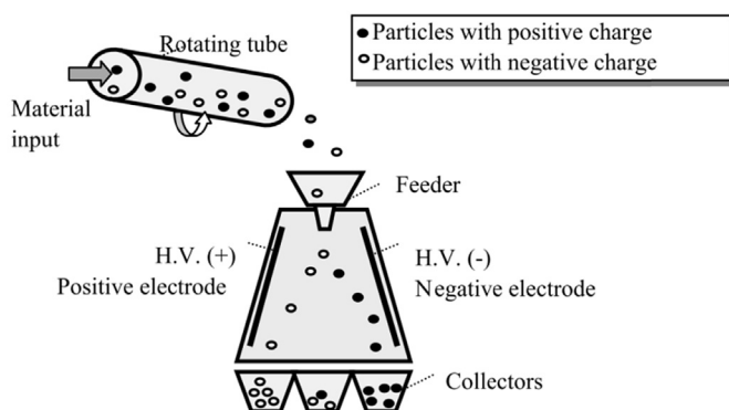
Fig. 5. Schematic representation of the Tribo electric separation [18].
