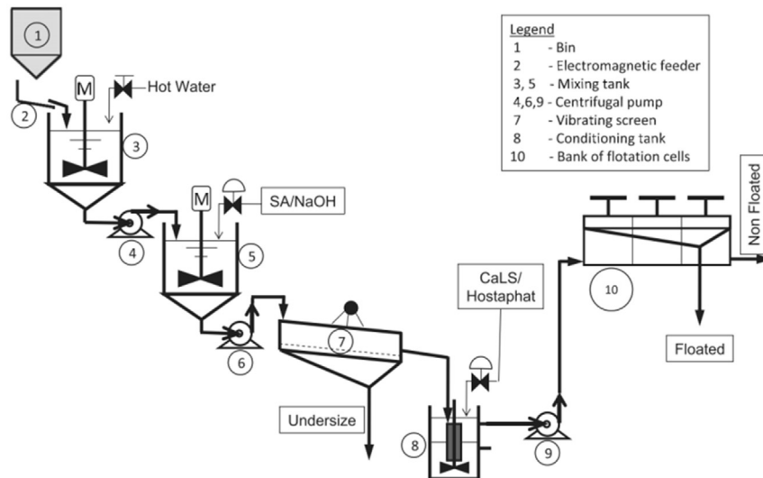
Fig. 6. Basic Process involves in froth flotation method Carvalho et al. [29].
