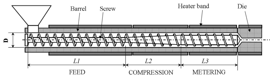
Fig. 10. Schematic of single screw extruder Covas and Gaspar-Cunha [30].
