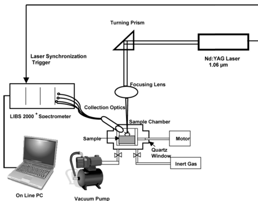
Fig. 4. Schematic of the LIBS experimental setup applied for the analysis of plastic samples, [51].
