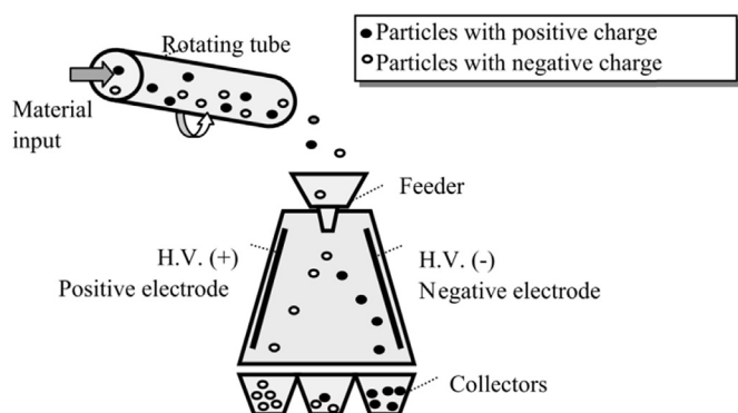
Fig. 5. Schematic representation of the Tribo electric separation [18].
